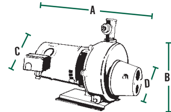
Overall Length "A" Overall Height "B" (without Regulating Valve) Overall Width "C" (with Pressure Switch) Overall Width "D" (without Pressure Switch) *See table to left for dimensions.
